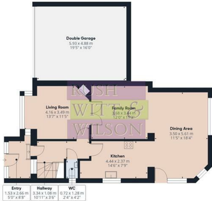
Floor 0 Building 1
